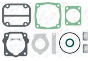
RK.01.046.21 Repair Kit
