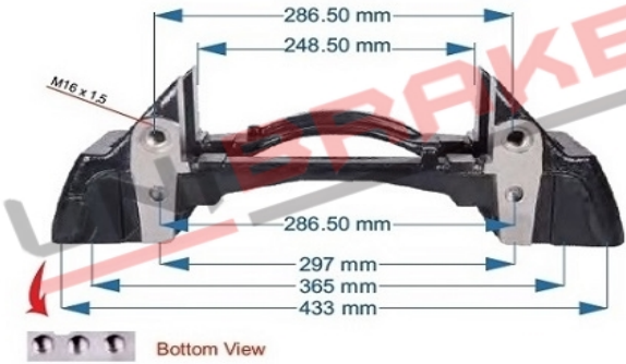
5818 / Caliper Carrier / B AXLE KNORR CARRIER
