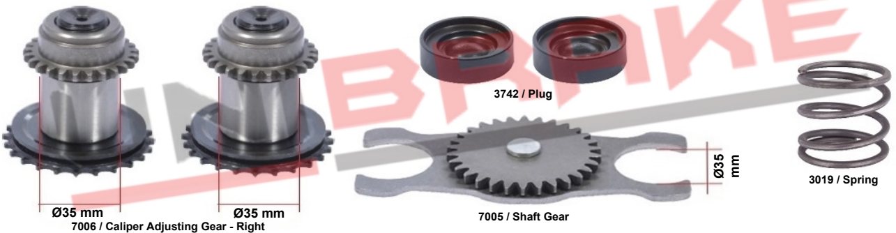
7008-1 / Caliper Adjusting Gear Set - Right ELSA 1 Type
