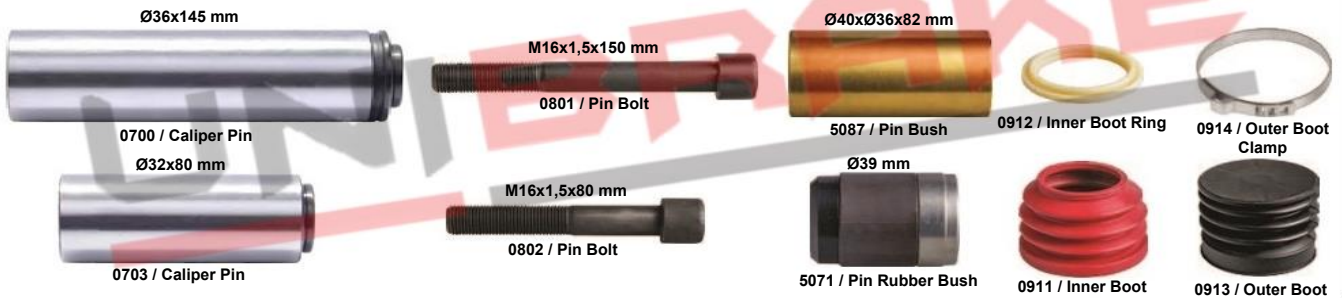
5091 / Caliper Pin Boot & Cap Set SB5 / SB6 / SB7 / SB7 Radial Type KNR: II350470061 / MB: 001 420 6683 / MN: 81.50822.6005
