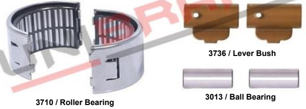
7170 / Caliper Bearing Set D DUCO / ELSA 2 Type MERITOR: SJ4098 / VOLVO: 3092261 / CMSK.98.3
