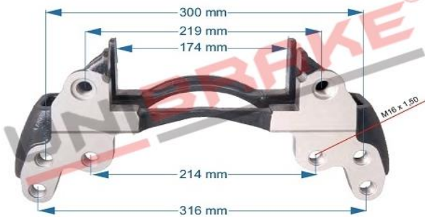
5820 / Caliper Carrier / MB ATEGO KNORR CARRIER
