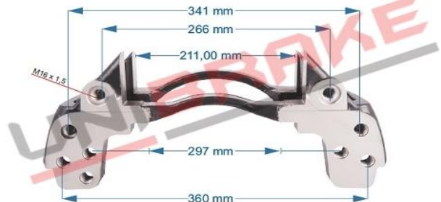
5831 / Caliper Carrier / IVECO TRUCK LEFT KNORR CARRIER KNORR: K002313
