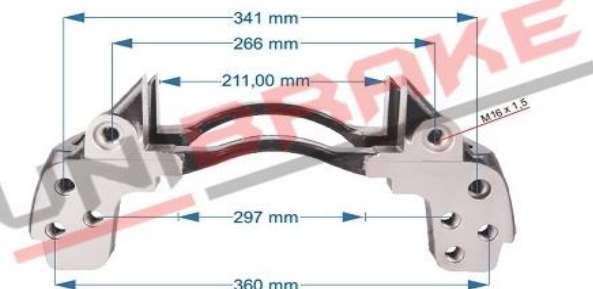
5830 / Caliper Carrier / IVECO TRUCK RIGHT KNORR CARRIER KNORR: K002314
