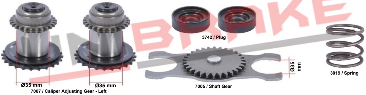
7008 / Caliper Adjusting Gear Set - Left ELSA 1 Type
