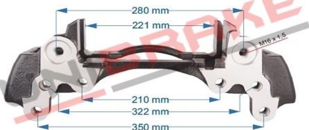
6821 / Caliper Carrier / MB AROCS REAR - RIGHT WABCO CARRIER 640.915.745.4 / MB: 000 423 2206
