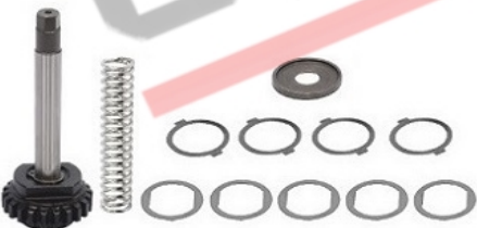
7061 / Caliper Adjusting Mechanism
