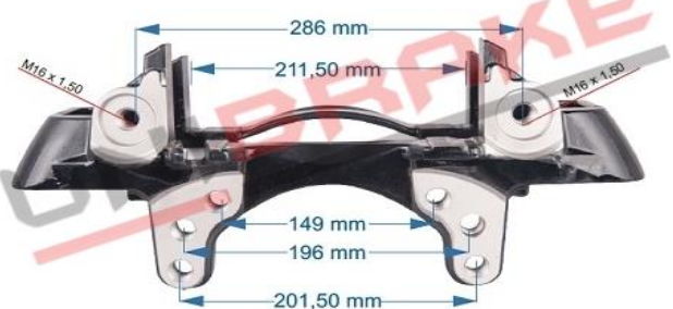
6820 / Caliper Carrier / SCHMITZ TRAILER - LEFT WABCO CARRIER
