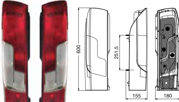
Rear Combination Lamp (without Socket) Arka Kombinasyon Lambası (Soketsiz)
