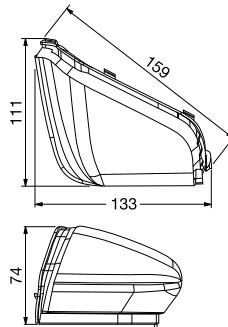
Outside Mirror-Indicator Lamp (With Bulb) Kapı Aynası Sinyal Lambası
