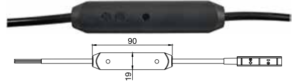
Order No: QPP171 Yan İşaret Kontrol Sistemi Side Marker Control Gear
