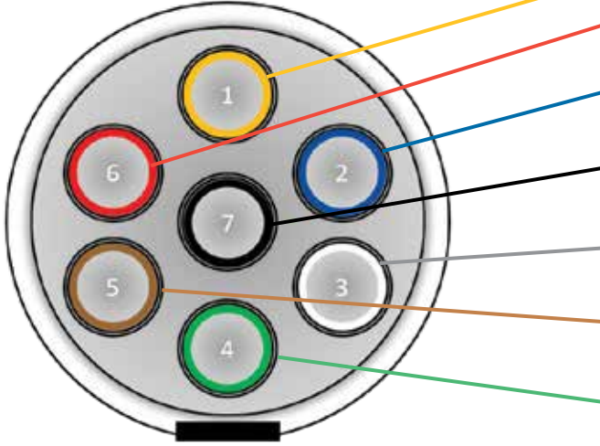
Inner View of Plug
