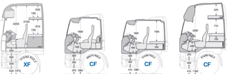
1 Super Space Cab 2 Day Cab 2 Sleeper Cab 3 Space Cab
