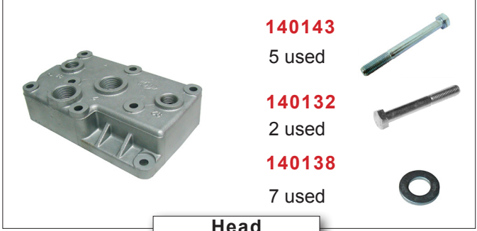
Head
