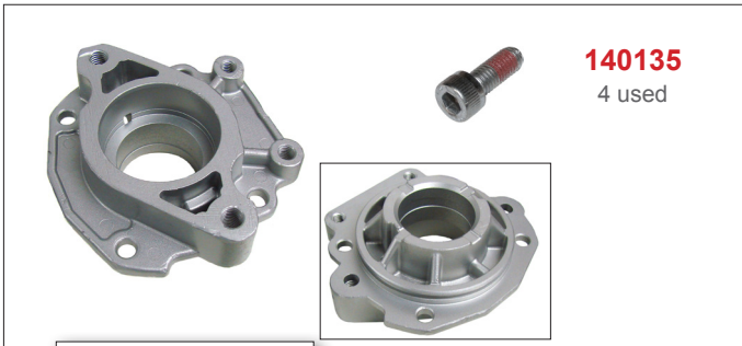
End cover
