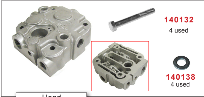
Head
