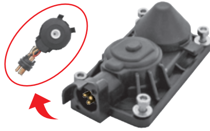
MTX-5279 Cover With Sensor (MAN) Pokrywa plastikowa z pot.
