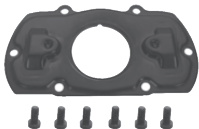
MTX-6212 Mechanism Cover Pokrywa dolna zacisku
