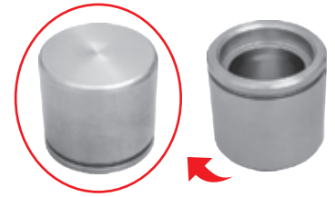
MTX-4015 Piston - F/B (68x63,5 mm) Tłok ham. (68x63,5 mm)
