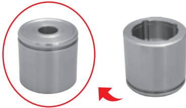
MTX-4007 Piston - H/B (68x63,5 mm) Tłok ham. (68x63,5 mm)
