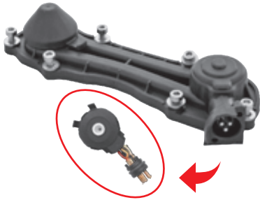
MTX-5284 Cover With Sensor (MAN) Pokrywa plastikowa z pot.
