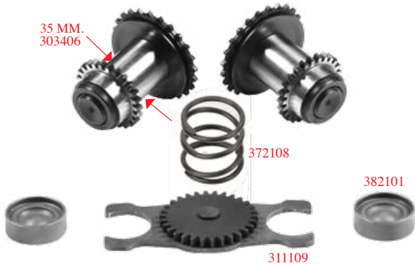
301401 > DİŞLİ SETİ-R / GEAR SET -R-
