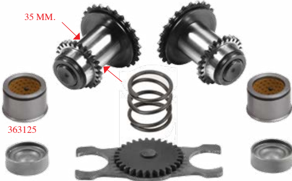
301410 > DİŞLİ SETİ-R / GEAR SET -R-
