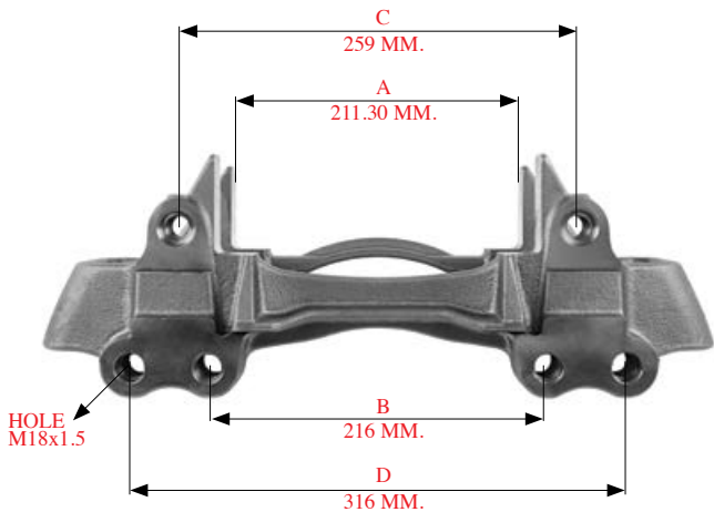
490101 > HLDX MODUL T BALATA TAŞIYICI HLDX MODUL T CARRIER
