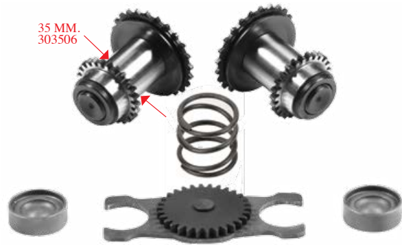
301501 > DİŞLİ SETİ-L / GEAR SET -L-
