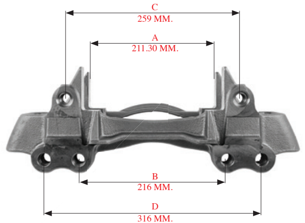
490101 > HLDX MODUL T BALATA TAŞIYICI HLDX MODUL T CARRIER
