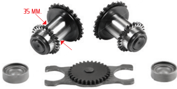
301401 > DİŞLİ SETİ-R / GEAR SET -R-
