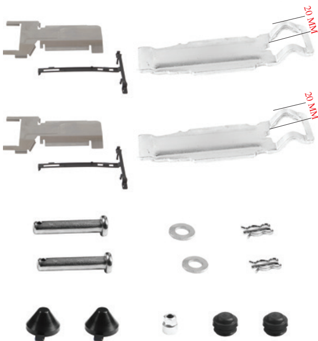
111112 İPAT TUTUCU TAMİR TK. BRAKE PAD RETAINER KIT
