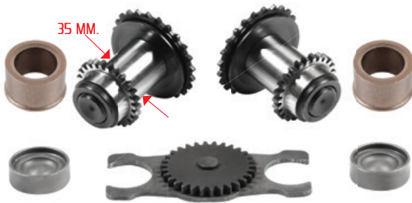
301410 > DİŞLİ SETİ-R / GEAR SET -R-
