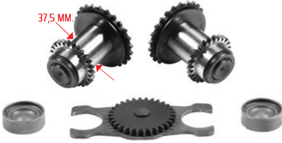
301402 > DİŞLİ SETİ-R / GEAR SET -R-
