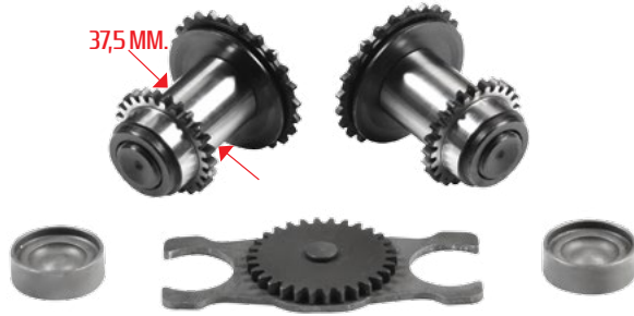
301402 > DİŞLİ SETİ-R / GEAR SET -R-
