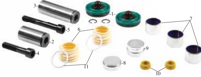
252112 TOZ LASTİK VE PERNO TAKIMI / CALIPER PIN & DUST RUBBER SET
