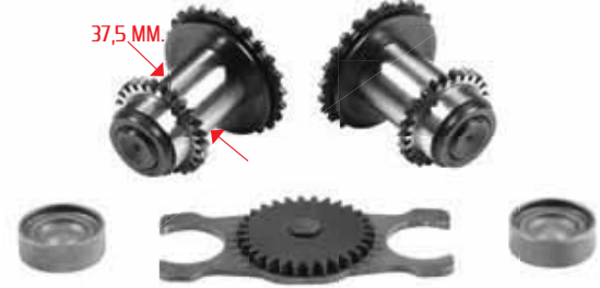
301502 > DİŞLİ SETİ-L- / GEAR SET -L-
