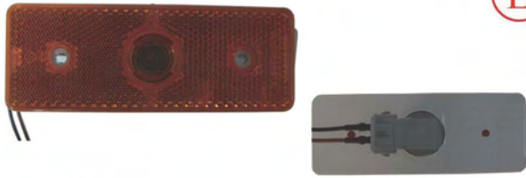
TD03-50-017 BENZ ACTROS SIDE LAMP SIZE:120×45mm SCREW HOLE:75mm
