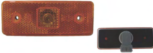
TD03-50-019 BENZ ACTROS SIDE LAMP 24V 3W OEM NO. 0005443711 SIZE:110×42mm
