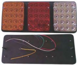
TD05-63-065 UNIVERSAL TAIL LAMP WITH 60 LED SIZE:330×140mm SCREW HOLE:306mm
