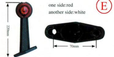
TD06-68-006 (OLD:TD03-63-006) MARKER LAMP LED
