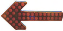
TD24-68-020 (OLD:TD05-63-120) UNIVERSAL REAR TURNING SIGNAL LAMP WITH 400 LED SIZE:600×270×100mm
