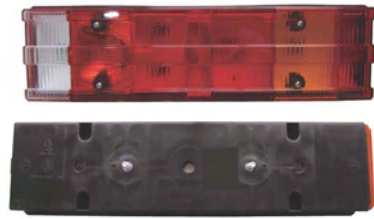
TD02-50-026 BENZ SPRINTER PICK UP AFTER 2006 REAR LAMP OEM NO.0025445503,0025445403 0025445603,0025447203 LANCE: A0025444790
