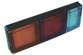
TD23-68-041 UNIVERSAL TAIL LAMP WITH 140 LED SIZE:425×156×46mm
