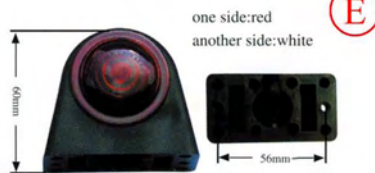
TD06-68-008 (OLD:TD03-63-008) MARKER LAMP LED
