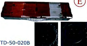
TD-50-020B BENZ ACTROS TAIL LAMP WITH PLUG OEM NO.0015405770,0015405870 LANCE 0025441290,0025441690
