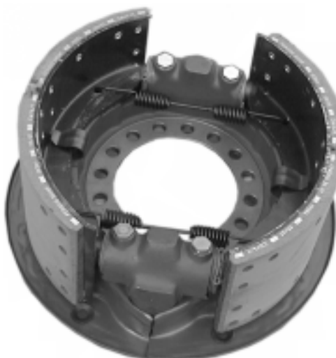
Assale posteriore Rear Axle
