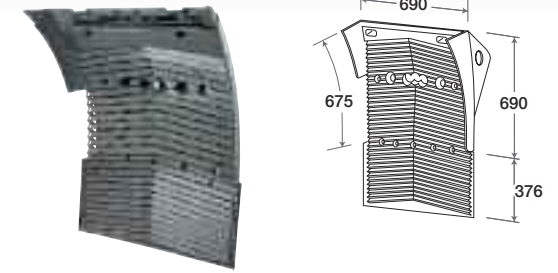
H. 376 TGX/528 O.E.M. 81664106630 TGX/529 O.E.M. 81664106629
