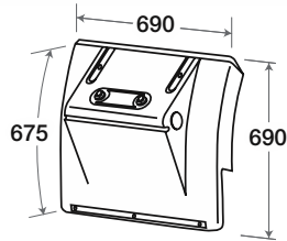
TGX/532 O.E.M. 81664106631 TGX/533 O.E.M. 81664106626
