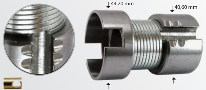
AYAR MEKANİZMA DİP LİSİ SAĞ BRAKE ADJUSTING MECHANISM GEAR RIGHT
