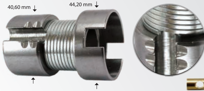
AYAR MEKANİZMA DİP LİSİ SOL BRAKE ADJUSTING MECHANISM GEAR LEFT
