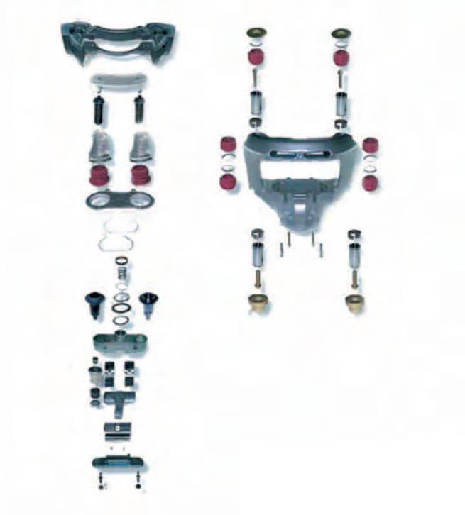
MARK IV BB 22 Type Caliper
