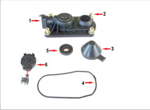
Caliper Plastic Cover (with sensor)
