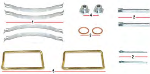
Caliper Pad Retainer Repair Kit
