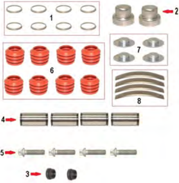
Caliper Guide & Seals Repair Kit
