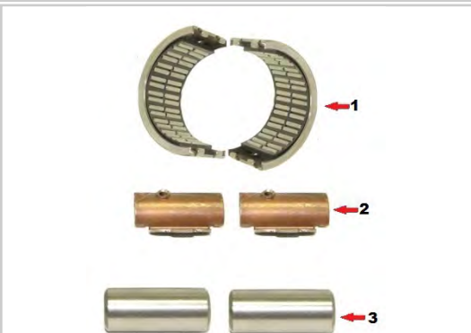
Caliper Half Bearing Repair Kit (Axial) SJ4112
