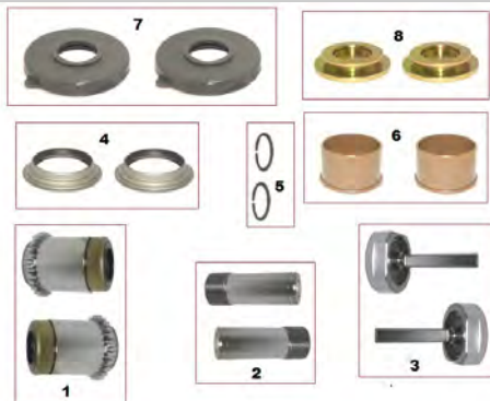
Caliper Adjuster Tappet Repair Kit (Left) MCK1236
