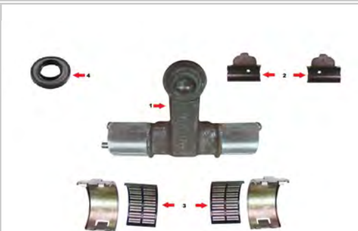
Caliper Lever Repair Kit (Axial - Left) SJ4096
