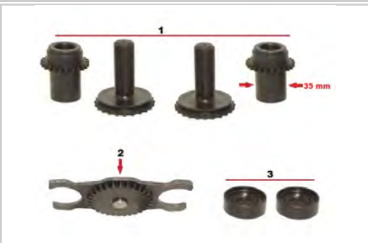
Caliper Tappet Adjusting Mechanism (Right)
