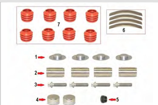
Caliper Guide & Seals Repair Kit
