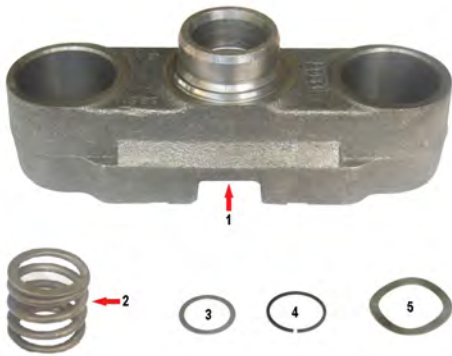
Caliper Bridge Assembly Repair Kit
