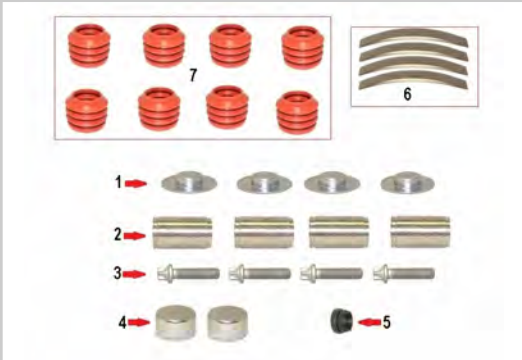
Caliper Guide & Seals Repair Kit
