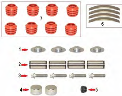
Caliper Guide & Seals Repair Kit
