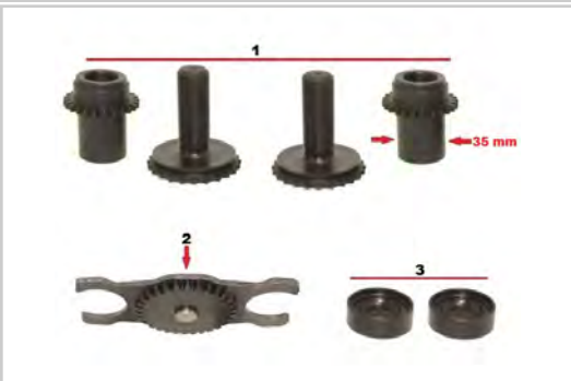
Caliper Tappet Adjusting Mechanism (Left)
