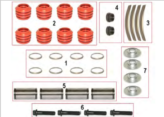
Caliper Guide & Seals Repair Kit
