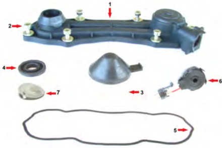
Caliper Sensor Cover (2 cables inside)
