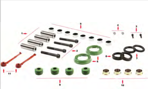
Caliper Guides & Seals Repair Kit 12 999 729
